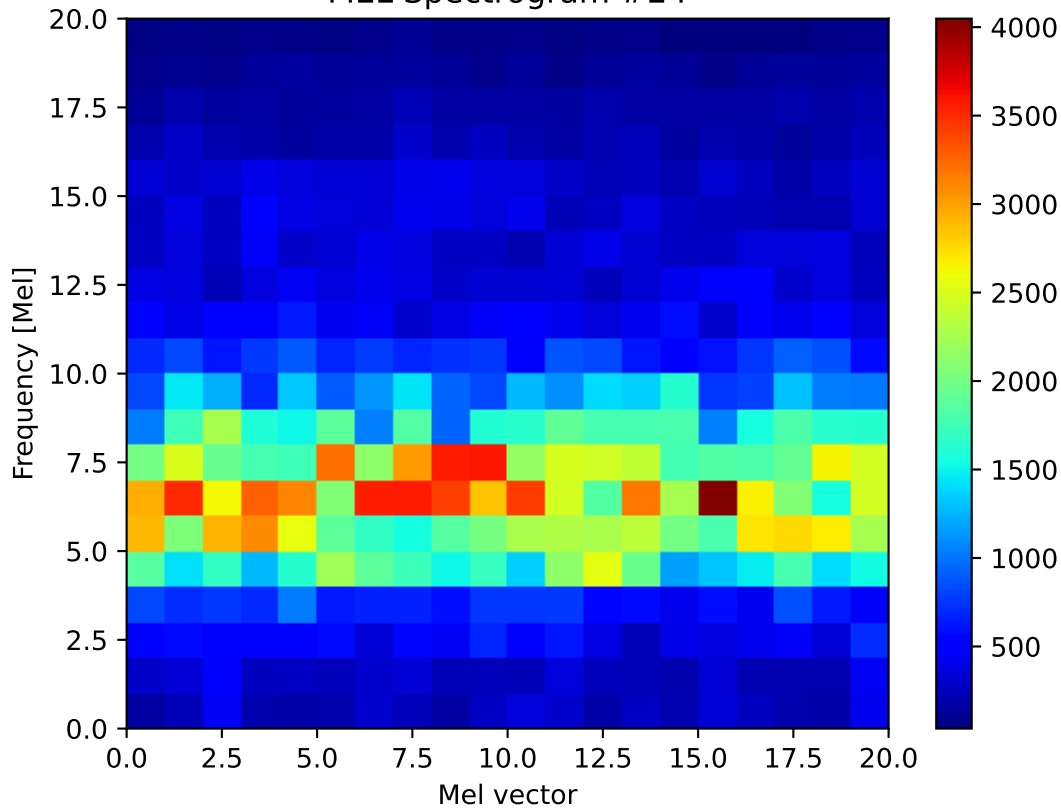
MEL Spectrogram #24
